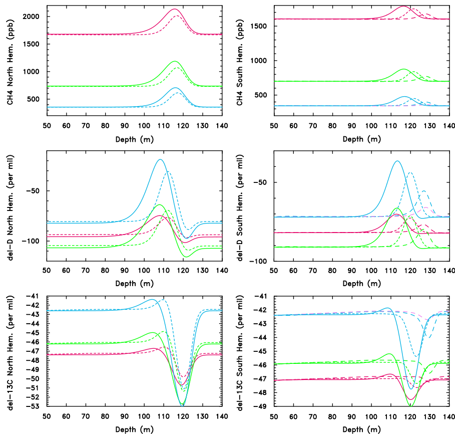
Fig. 4. CH 4 , δD CH 4 and δ 13 C CH 4 signals in ice cores following a 4000 Tg CH 4 pulse emission at 65°N in March. Black(Red online): present conditions, dark grey(green online): PIH, light grey(blue online): LGM. "Acc" values below are accumulation rates in cm w eq yr -1 . Left panel: Arctic sites (Devon Island: continuous lines, acc=30, North GRIP: short dashed lines, acc=17); right panel: Antarctic sites (Berkner Island: continuous lines, acc=13, Dronning Maud Land: short dashed lines, acc=7, Dome C: long dashed lines, acc=3.6. the lightest grey lines(purple lines online) show the Dome C results with reduced (LGM) temperature and accumulation rate (acc=1.2). Note the different vertical scales.
