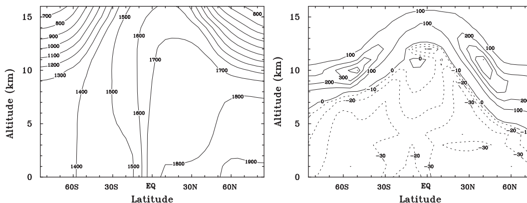
Fig. 2. Methane concentration (ppb, left panel) and OH difference from the equilibrium field (%), 1 yr after an emission from clathrates (4000 Tg CH 4 in one time step, at 65°N in March, in LGM climatic conditions).
